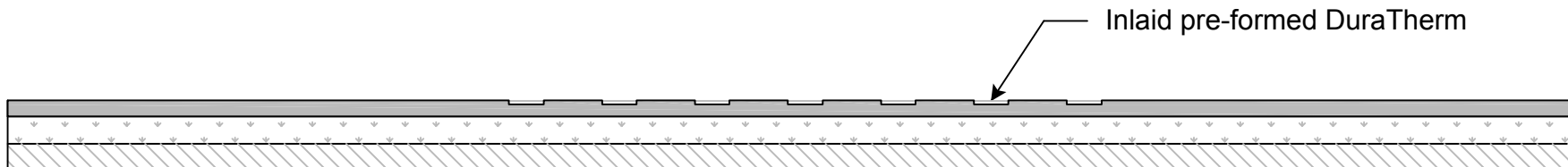
DuraTherm Cross Walk - contiuous asphalt
