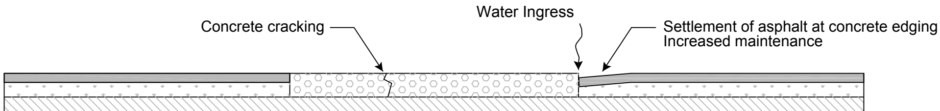
Stamped Concrete Cross Walk - after a few winters
