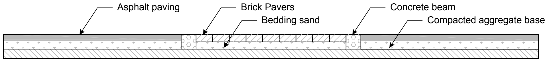
Brick Paver Cross Walk - New
