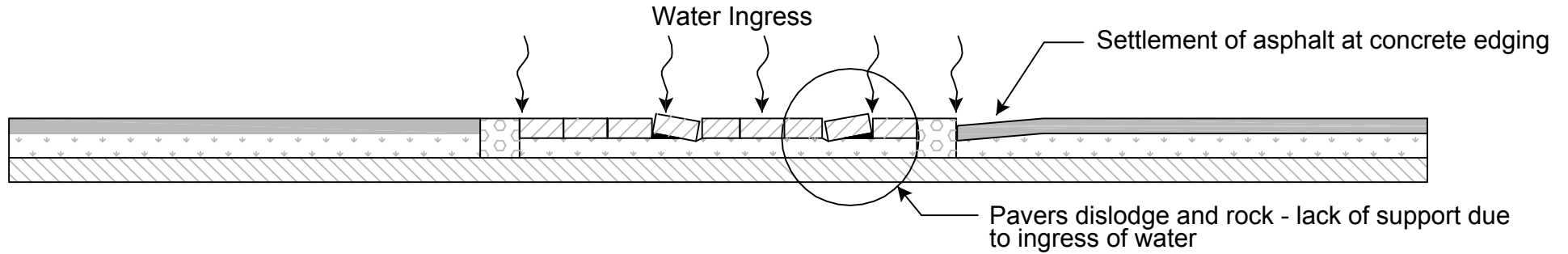
Brick Paver Cross Walk - after a few winters
